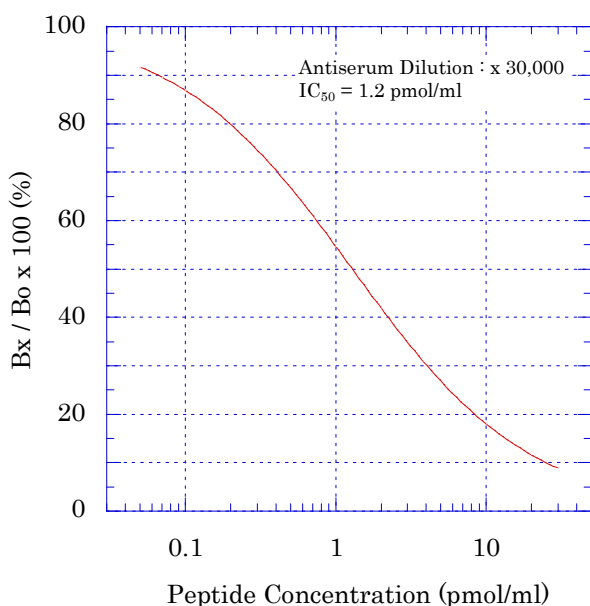
Standard Curve of Galanin (Rat)
