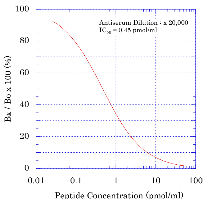
Standard Curve of CGRP (Human)
